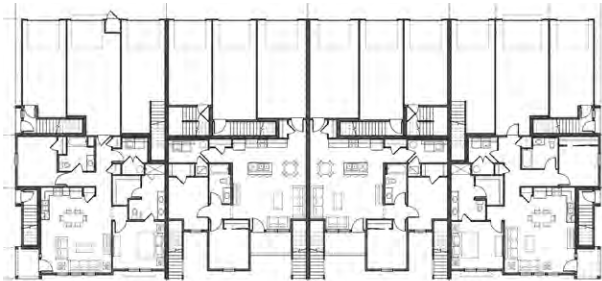
12-PLEX MAIN LEVEL
