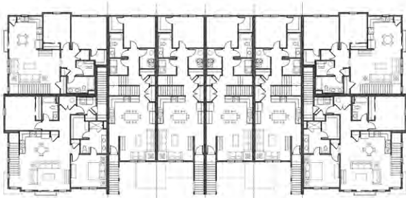
12-PLEX UPPER LEVEL
